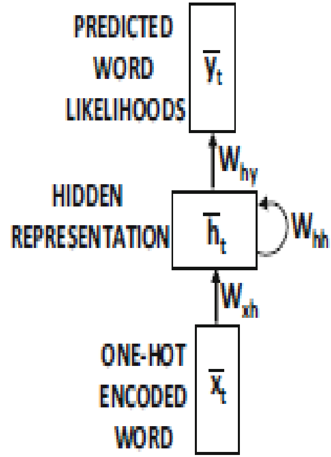
(a) RNN
